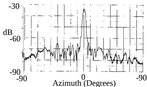
Fig.8: Radiation pattern of the boresight beam in the azimuth direction
